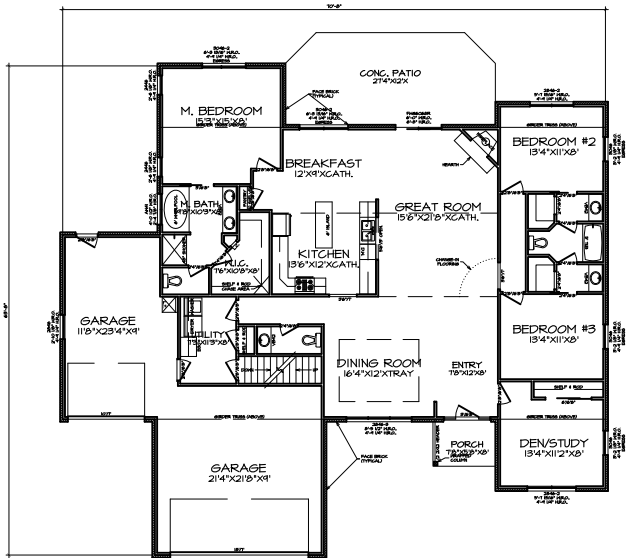
FIRST FLOOR PLAN A-1
