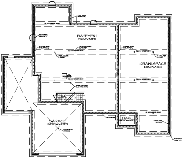
FOUNDATION PLAN A-1
